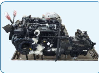
ENGINE Volvo Eicher make CEV BS V, 74 hp Diesel Engine, High Pressure Common Rail System Technology, Turbo Charged Water Cooled, ECU Control Engine Management.
